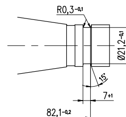
Cone com ranhura anular MAHO Taper shanks with MAHO ring groove
